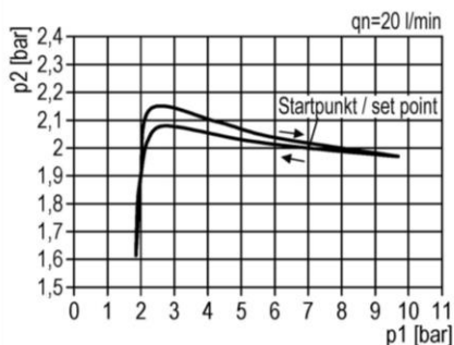
Hysteresis
