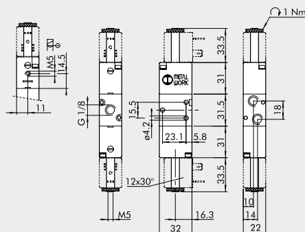
BISTABIL 3/2, 1/8"
