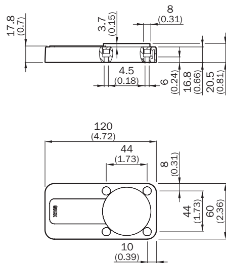
Dimensional drawing Actuator
