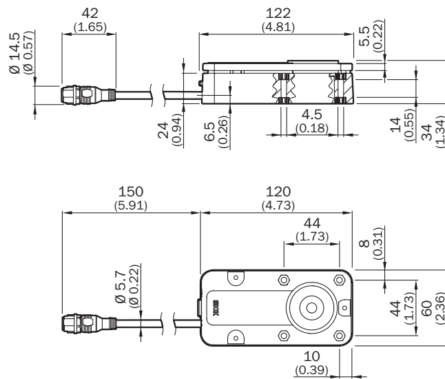
Dimensional drawing Sensor with M12 male connector
