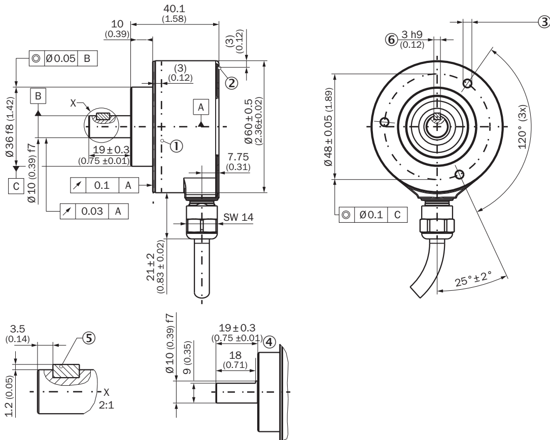
Dimensional drawing Solid shaft, face mount flange, radial cable
