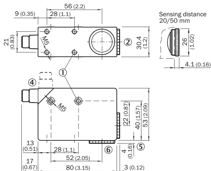
Dimensional drawing LUT9x-x2xxx, light emission: long and short side, exchangeable
