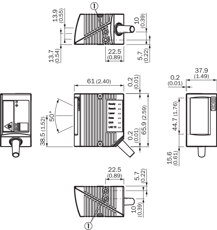
Dimensional drawing CLV62x Standard, front
