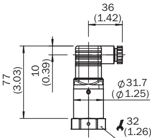
Dimensions in mm (inch)
