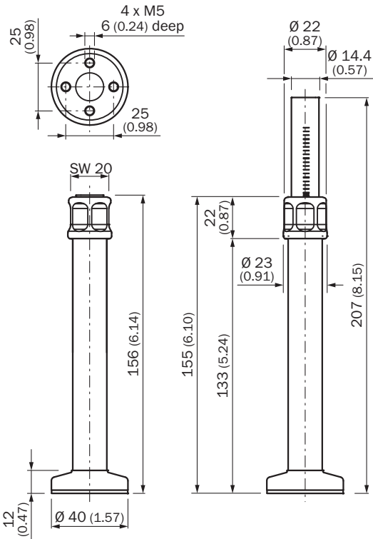
Dimensions in mm (inch)
