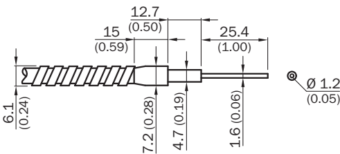
Dimensions in mm (inch)
