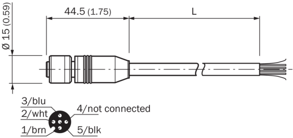
Dimensions in mm (inch)
