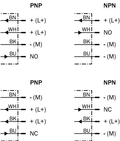
Connection diagram Cd-027
