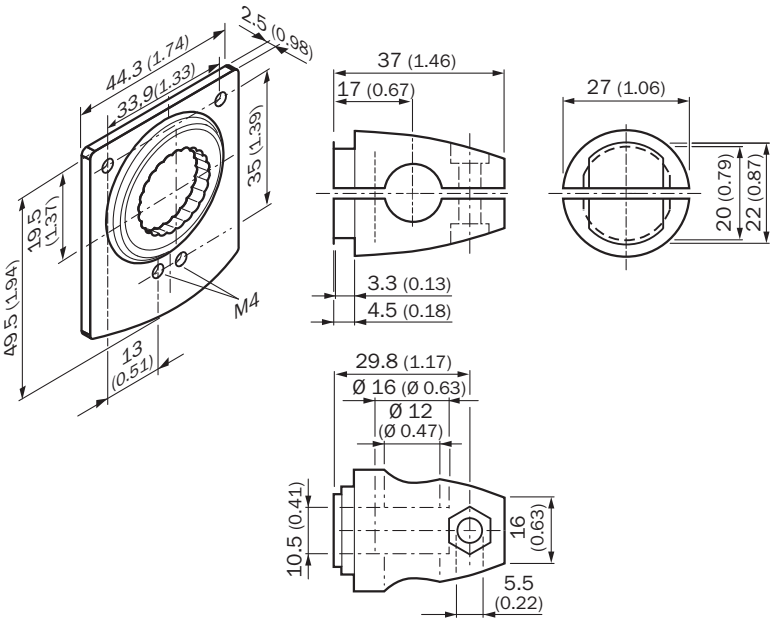
Dimensions in mm (inch)
