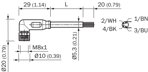
Dimensions in mm (inch)
