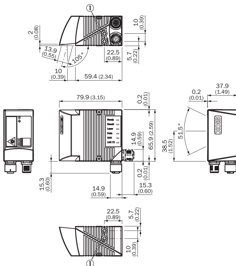
Dimensional drawing CLV62x Ethernet, side
