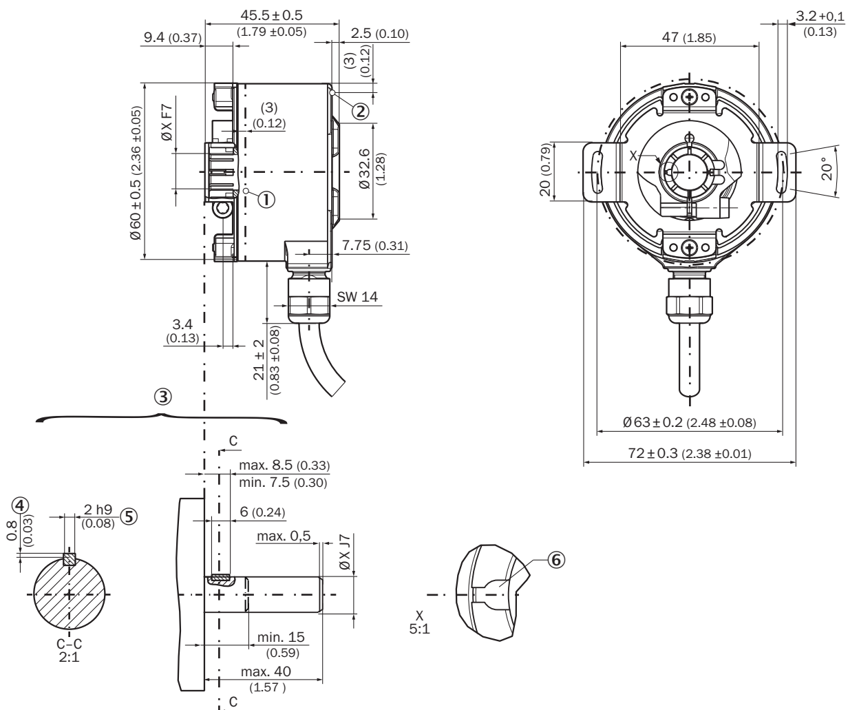
Dimensional drawing Blind hollow shaft, radial cable
