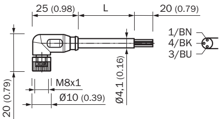
Dimensions in mm (inch)
