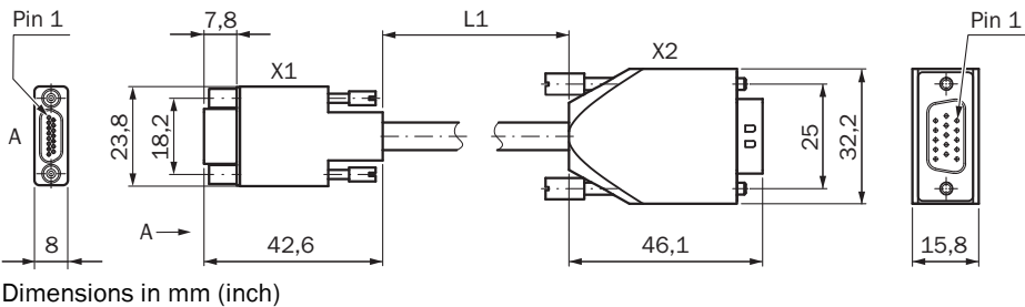
Dimensions in mm (inch)
