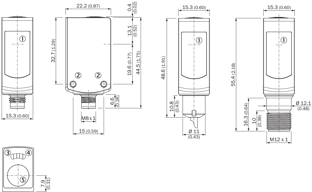
Dimensional drawing WL4S-3V, WLG4S-3V, with single teach-in button
