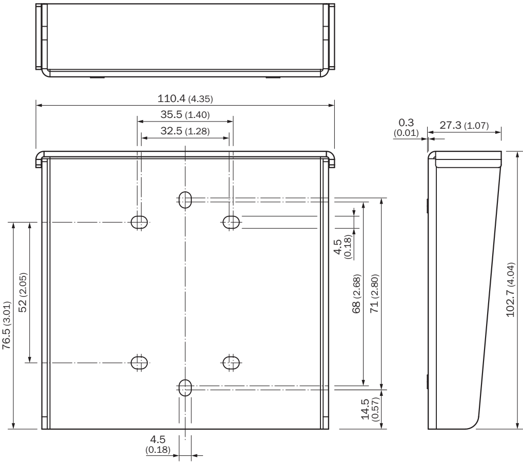
Dimensions in mm (inch)
