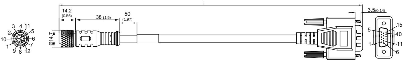
Dimensions in mm (inch)
