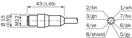
Dimensions in mm (inch)
