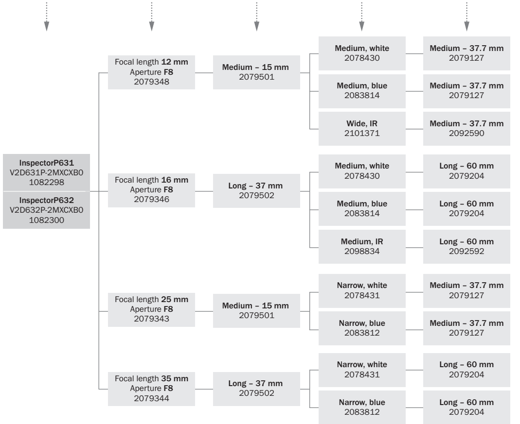
Spacer screws and illumination connector
