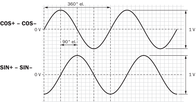
Diagrams Signal SIN/COS after differential generation
