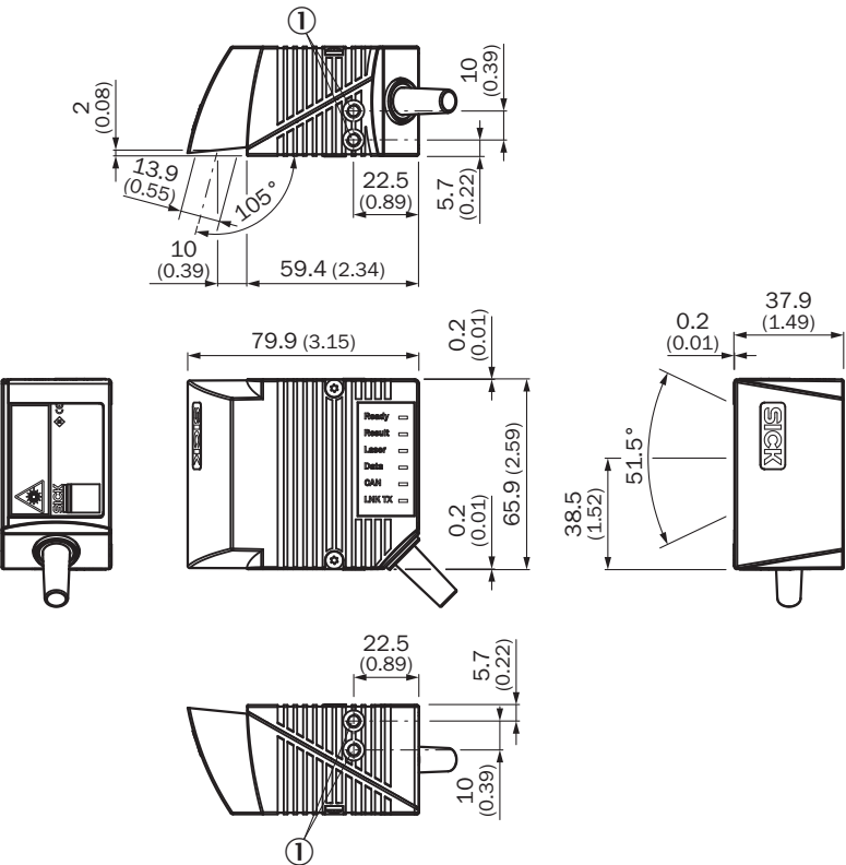
Dimensional drawing CLV62x Standard, side
