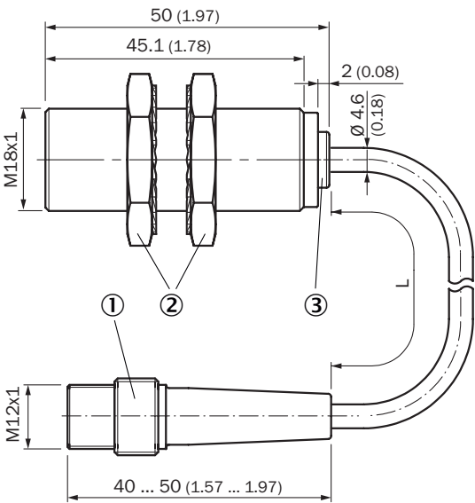
Dimensional drawing IMB18 standard, cable with male connector, flush
