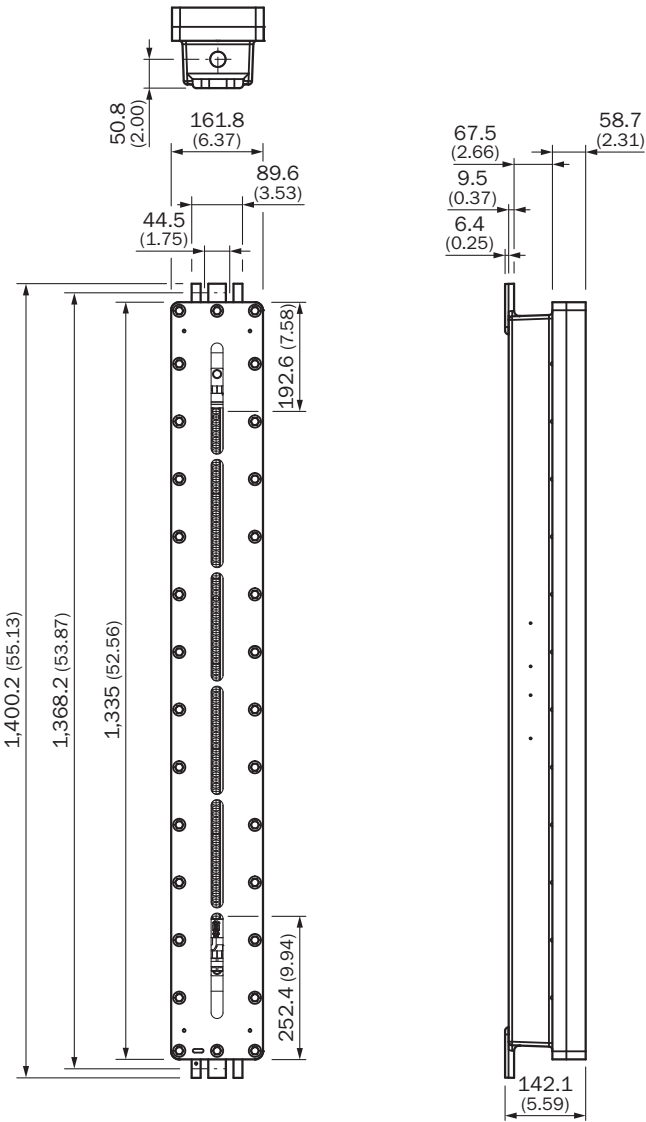
Dimensional drawing C4000 Advanced Ex, 900 mm
