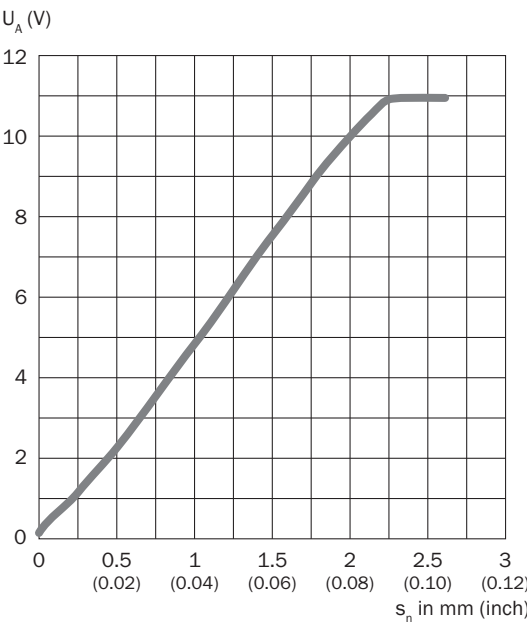
Response diagram Output voltage
