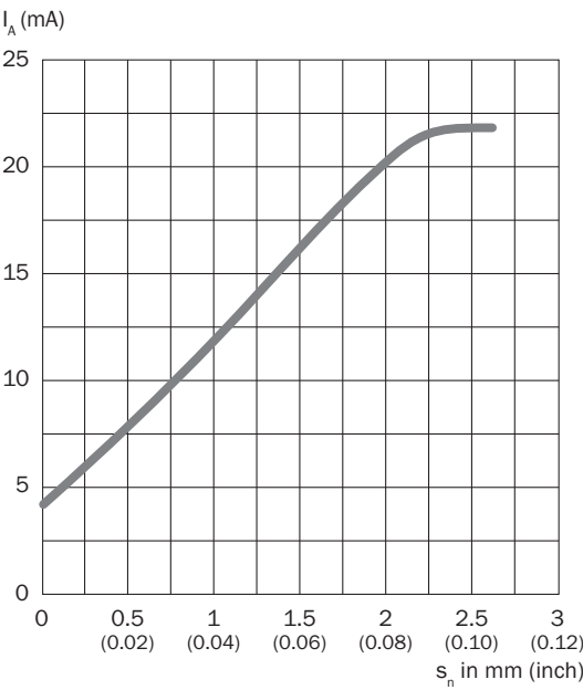
Response diagram Output current
