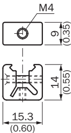
Dimensions in mm (inch)
