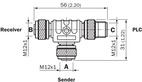
Dimensional drawing SBO-02F12-SM
