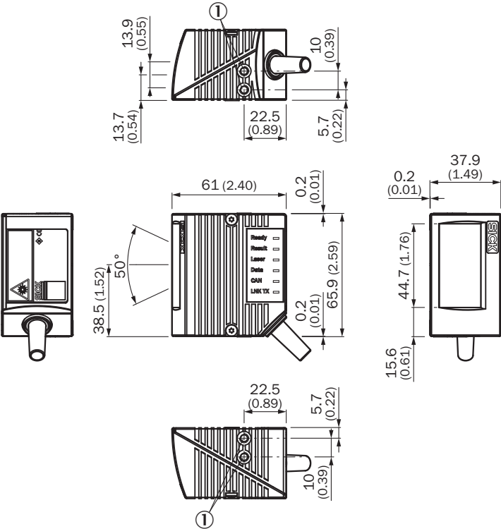
Dimensional drawing CLV62x Standard, front
