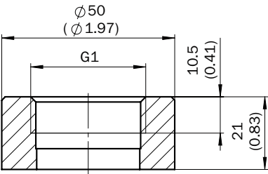
Dimensions in mm (inch)
