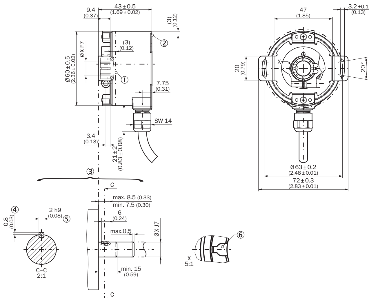
Dimensional drawing Through hollow shaft, radial cable
