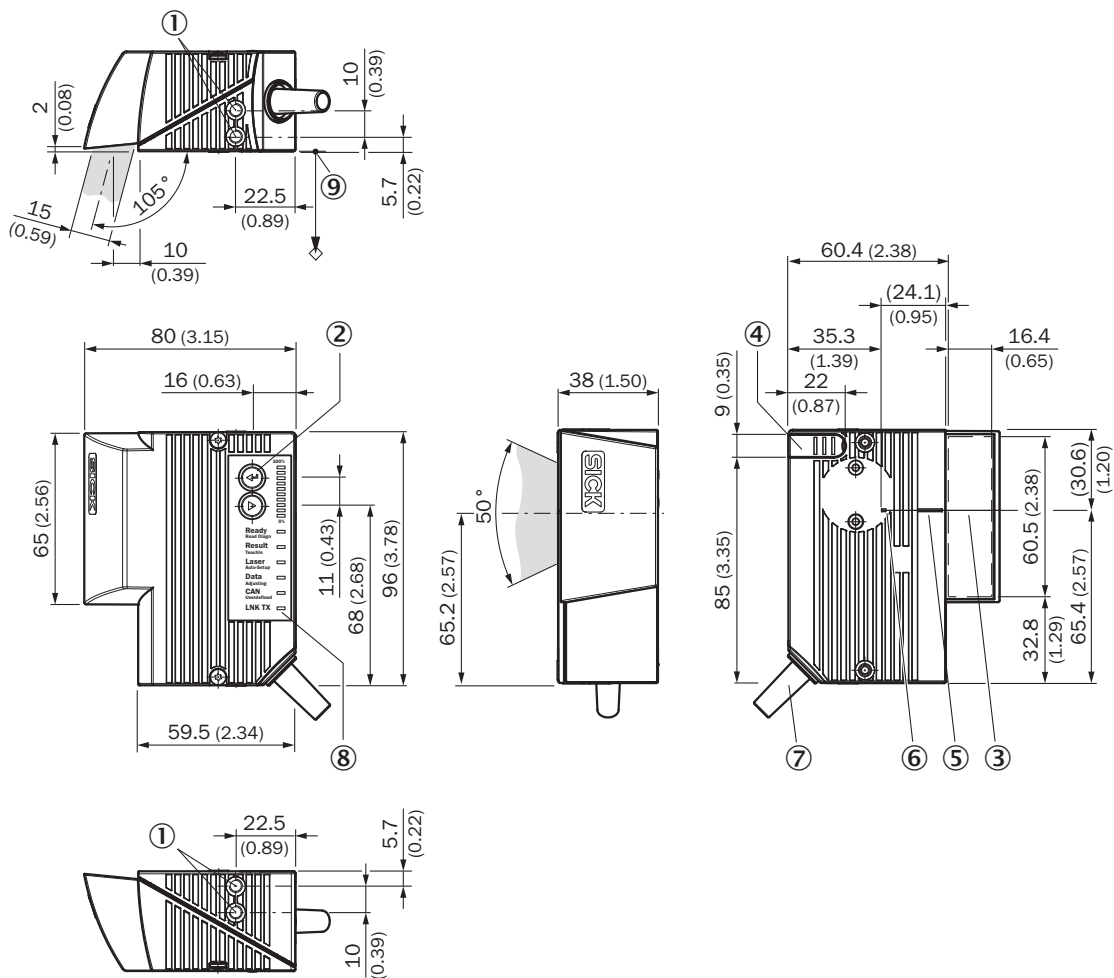
Dimensional drawing CLV63x/64x Standard, side
