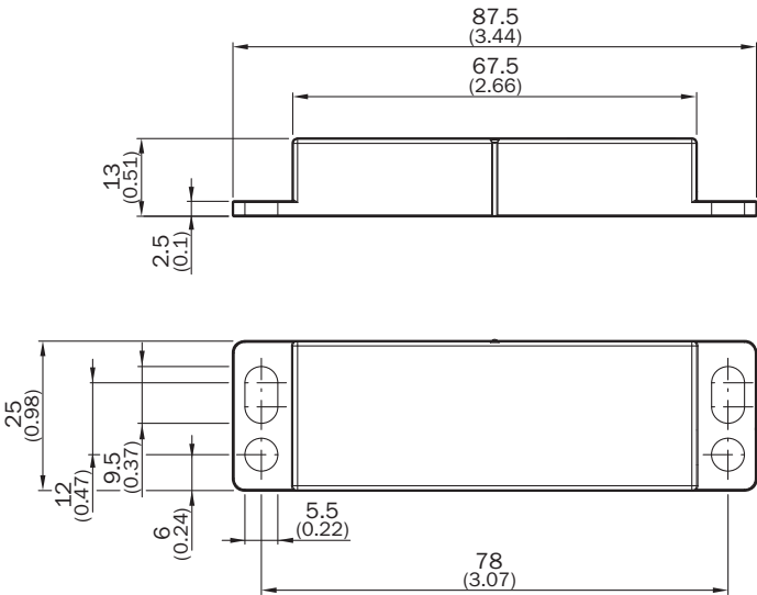
Dimensions in mm (inch)
