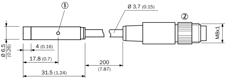
Dimensional drawing IHM06, short variant, non-flush, cable with male connector
