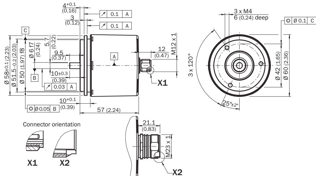
Dimensional drawing Servo flange, M12 and M23 axial male connector
