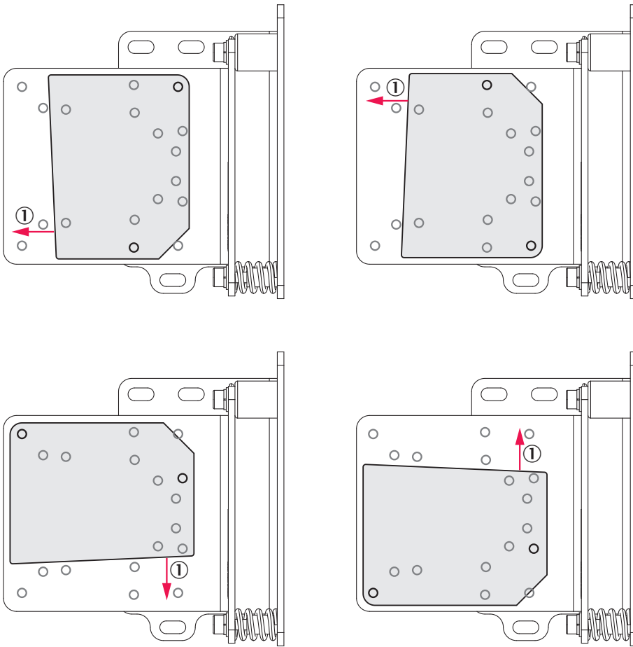
Mounting instructions for OD1000 ① sender
