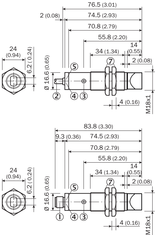
Dimensional drawing VTF180-2, VTE180-2, metal, radial
