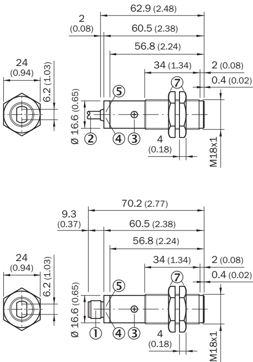
Dimensional drawing VL180-2, metal, axial
