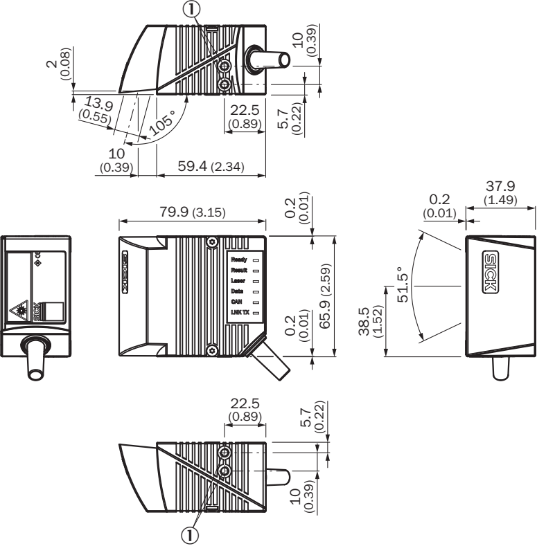
Dimensional drawing CLV62x Standard, side
