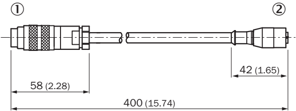
Dimensions in mm (inch) ① Connector M16, 8-pin ② male connector M12, 4-pin
