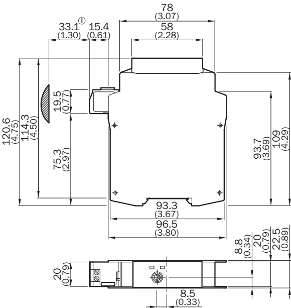
Dimensions in mm (inch) ① Approximate connector range
