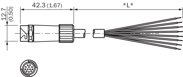
Dimensional drawing DOL-1212-G05M DOL-1212-G10M DOL-1212-G20M
