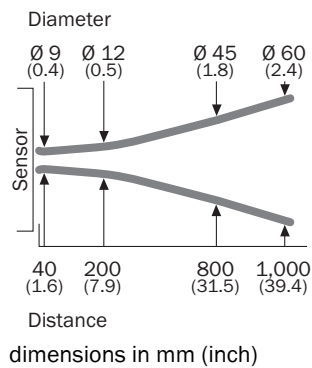
Light spot size GRTE18, 800 mm
