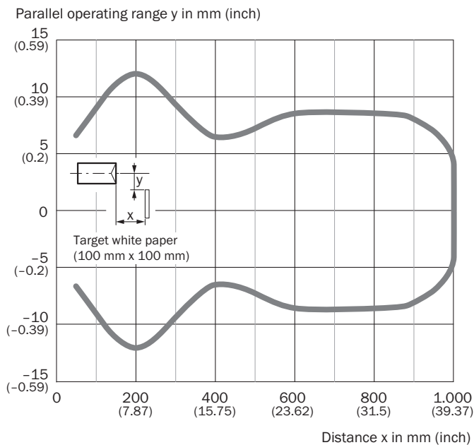
Response range GRTE18, 800 mm
