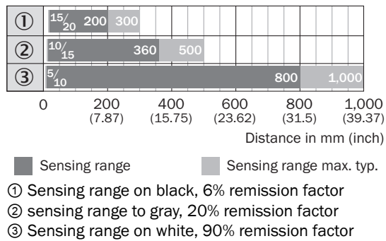
Sensing range diagram GRTE18, 800 mm
