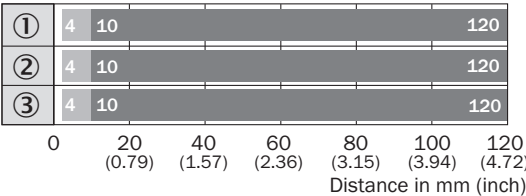
Sensing range diagram WTB4S-3, 120 mm
