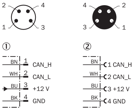
① male connector M8, 4-pin ② Cable with female connector, M8, 4-pin
