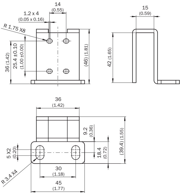
Dimensions in mm (inch)
