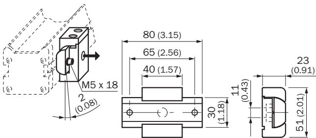
Dimensions in mm (inch)
