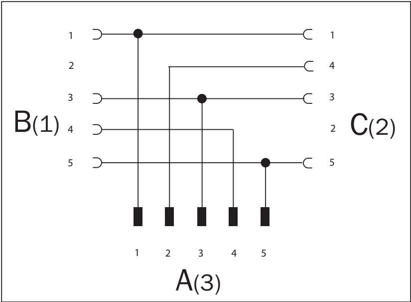
Connection diagram
