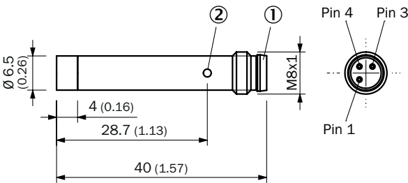
Dimensional drawing IHM06, short variant, non-flush, male connector
